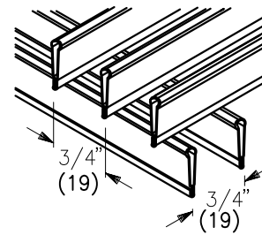
ADJUSTABLE DOUBLE DEFLECTION
